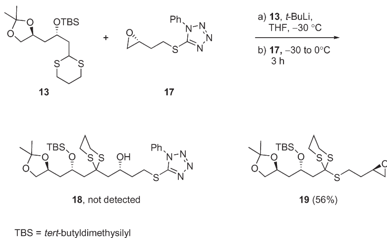
SCHEME 2 Sulfanylation of dithiane 13 by S-alkyl-N-phenylthioalkyltetrazole 17
