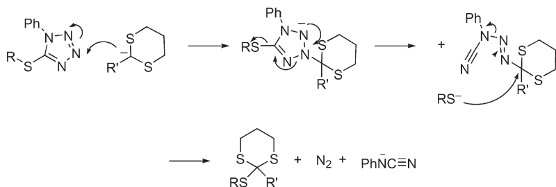
FIG. 2 A speculative mechanism for the sulfanylation
