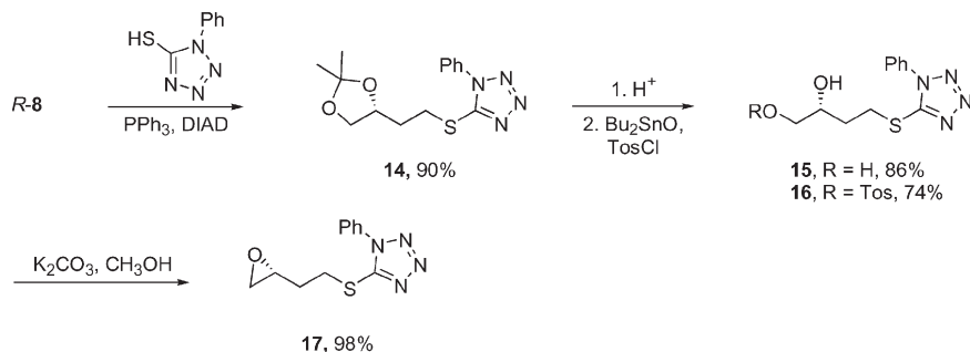
SCHEME 1 Synthesis of the precursors 13 and 17 for dithiane alkylation
