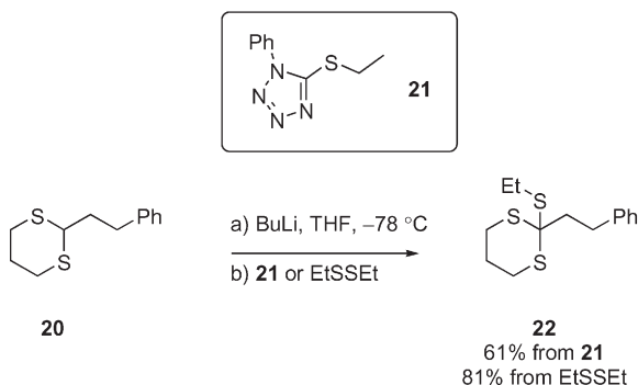
SCHEME 3 Simple model sulfanylations
